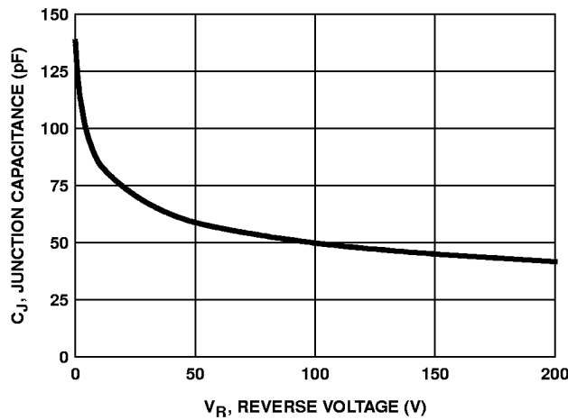
FIGURE 7. JUNCTION CAPACITANCE vs REVERSE VOLTAGE
