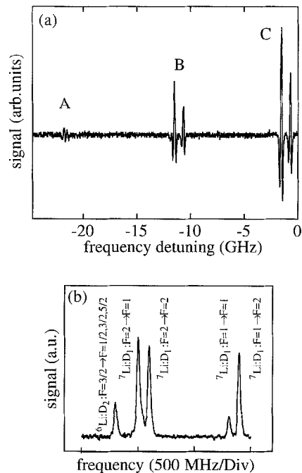
Fig. 3. Absorption spectrum of a lithium beam. The upper spectrum (a) shows a 24 GHz scan of the laser frequency. Due to the increase of the injection current, the laser intensity changes approximately by a factor of two during the scan. In order to eliminate this effect we have observed the second derivative of the absorption spectrum. The laser frequency is slightly modulated at 1 kHz and the second-harmonic of the modulation frequency is detected in the light transmitted through the lithium beam by means of a lock-in amplifier. The lines marked with A and C correspond to the D1 transitions of {}^6\text{Li} and D2 transitions of {}^7\text{Li} respectively. The lower scan (b) shows the line group B magnified.
