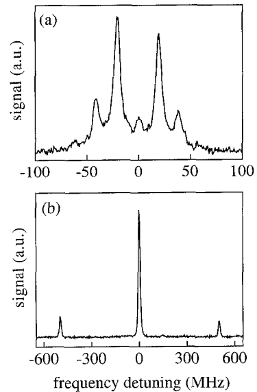
Fig. 4. Spectra of the laser output modulated at 20 MHz (a) and 500 MHz (b). The spectra are obtained by observing the transmission of a scanning Fabry-Pérot resonator (spectral resolution 10 MHz). We have used -13 dBm RF-power in (a) and 15 dBm in (b) respectively.
