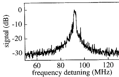
Fig. 2. Beat signal between two independent laser systems at 670 nm.
