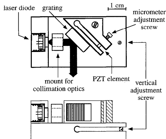
Fig. 1. Schematics of the mechanical setup of the grating-stabilized diode laser system.
