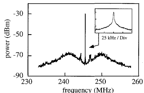
Fig. 6. Beat signal between the master laser and the slave laser with closed OPLL. A frequency span of 25 MHz was recorded with a resolution bandwidth of 1 kHz and a video filter bandwidth of 1 kHz. The increase in the noise level \pm 5 MHz from the center shows the noise sidebands of the stabilization loop. The inset shows a frequency span of 100 kHz, recorded with a resolution bandwidth of 1 kHz and a video filter bandwidth of 30 Hz. The width of the beat signal is limited by the resolution of the spectrum analyzer.
