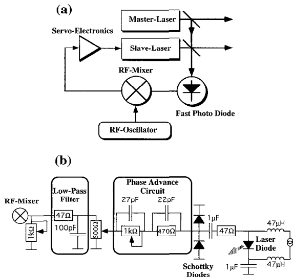
Fig. 5. (a) Schematics of the set-up for the optical phase locked loop (OPLL) between two independent lasers systems. The frequency of the master laser is stabilized to a Doppler-free resonance of the rubidium D2 line, using standard techniques. The frequency of the slave laser is stabilized by a heterodyne OPLL. (b) Electronic circuitry for the OPLL. The output signal from the RF-mixer is low-pass filtered (3 dB point at 34 MHz) to suppress the frequency of the local oscillator and its higher harmonics. A phase advance circuit then compensates for the delay with the error signal undergoes between the photodiode and the slave laser. The two Schottky diodes eliminate high frequency spikes that could damage the laser diode.
