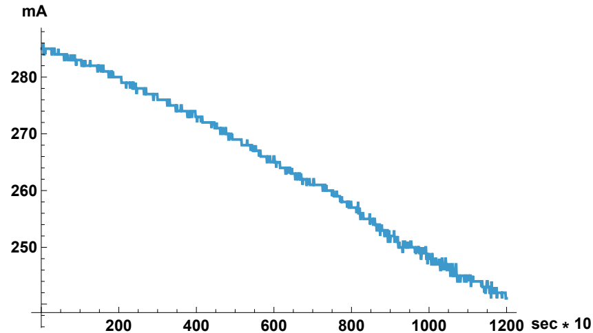
TEC current
