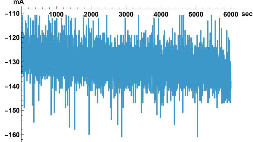
TEC current
