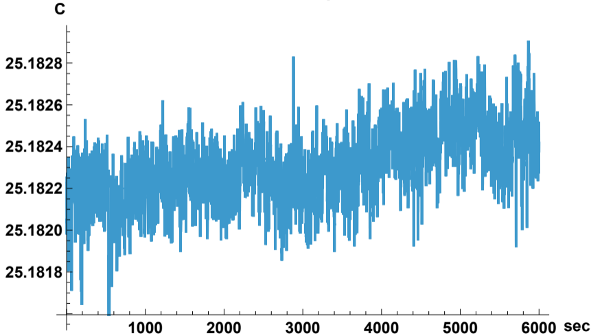
External Temperature
